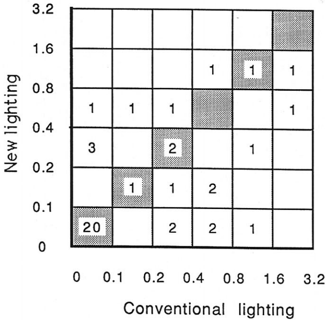
Figure 5 Scatterplot showing the weekly incidence of headaches under new and conventional lighting for the 42 subjects who experienced both conditions. The number in each cell indicates the number of subjects. There is a weak tendency for data to lie below the diagonal, suggesting a slightly greater susceptibility to headaches under conventional lighting
